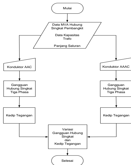
Gambar 2. Alur Penelitian
